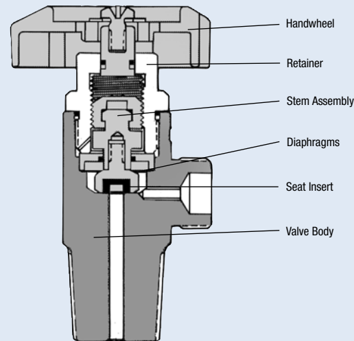
Tied-Diaphragm Valve (third generation)
