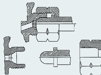
A typical bullet-nose connection.
