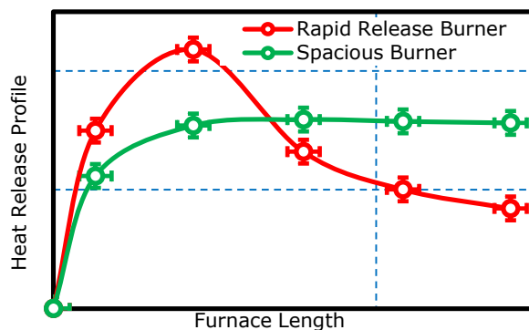
Figure 1: Heat release profiles for different types of Air Products oxy-fuel burners measured under controlled conditions in a test furnace
