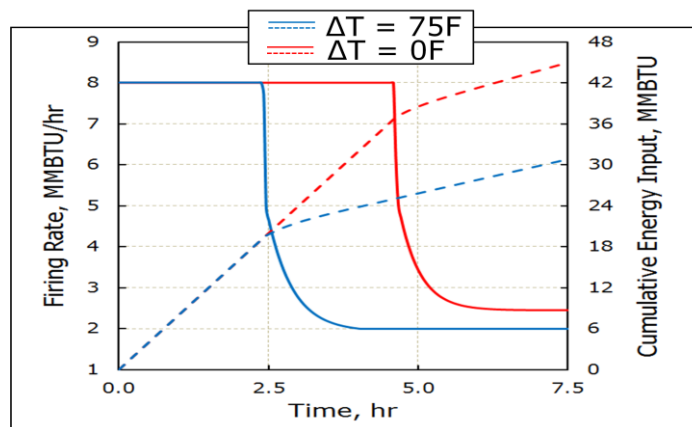
Figure 3: Illustration of firing rate and cumulative energy input into the furnace when the difference between control TC and steel temperature ( \Delta T ) is (a) 0 °F (when control TC matches the steel temperature) and (b) 75 °F (when control TC measures higher than the steel temperature).
