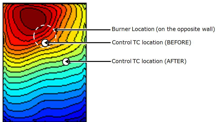
Figure 4: CLOP output ranking the locations for placement of control thermocouple for most effective control strategy. Red = worst location to Blue = best location.
